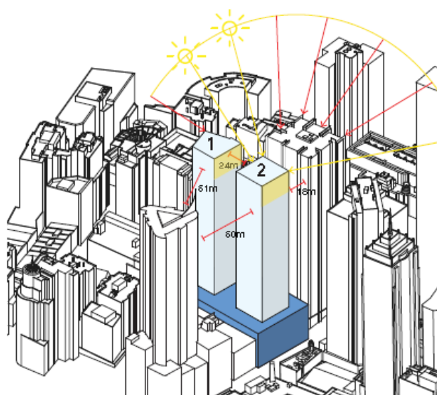
Daylight exposure
